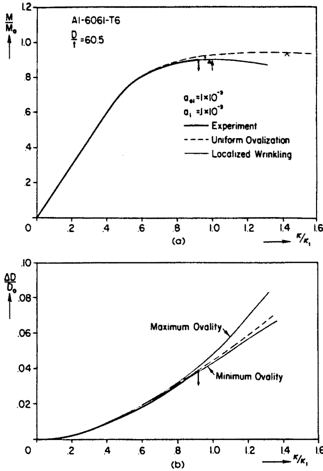
Fig. 15. Detailed comparison between experiment and predictions from analyses which include ripple localization ( D/t = 60.5 ): (a) moment curvature; (b) ovalization curvature.
